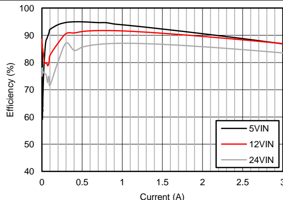
Figure 56. Efficiency at Room Temperature
