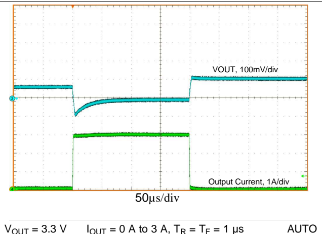
Figure 42. Load Transient
