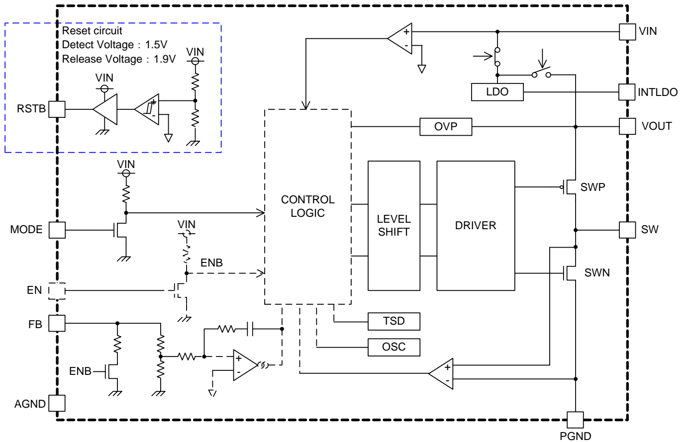
Figure 4. Circuit Block
