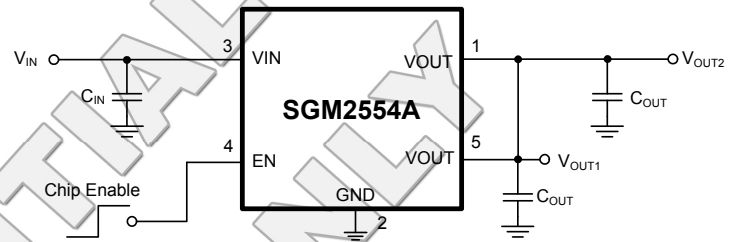
Figure 2. High-side Power Switch with Chip Enable Control
