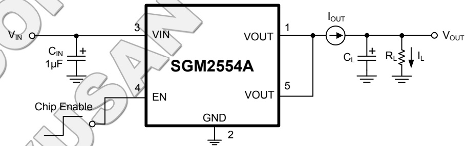
Test Circuit 3
