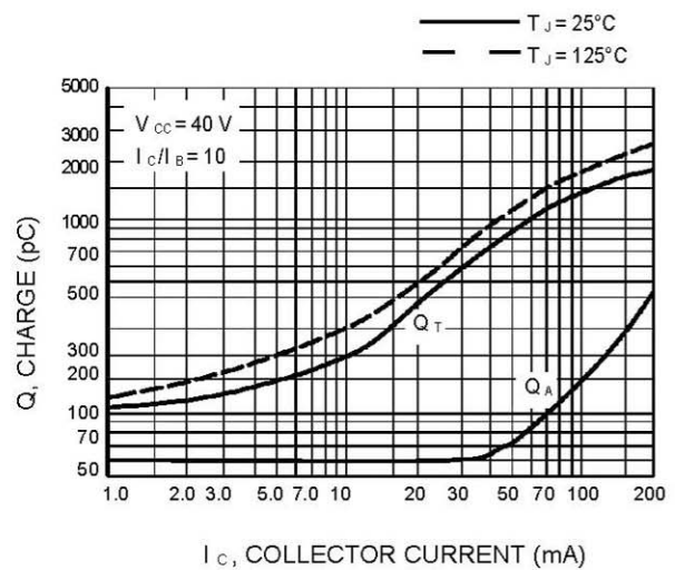
Figure 4. Charge Data
