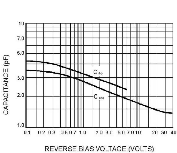
Figure 3. Capacitance
