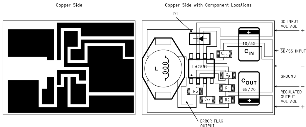
Figure 49. Typical Surface-Mount PCB Layout, Fixed Output (2X Size)
