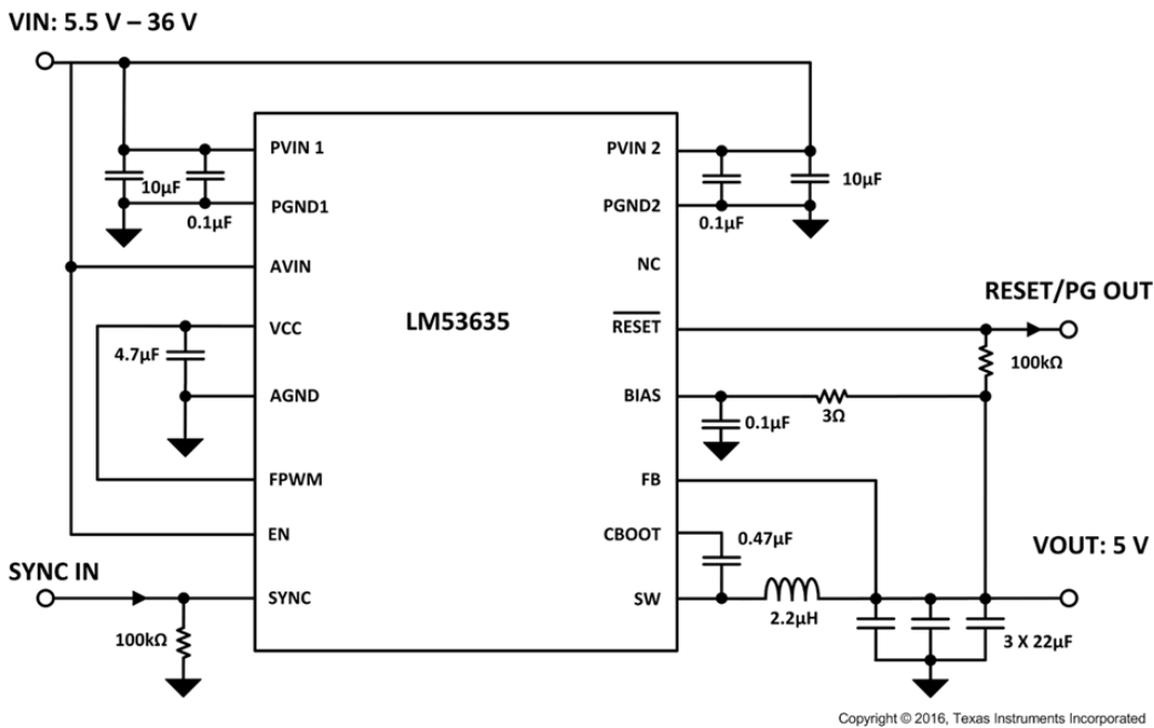
Figure 24. Fixed 5-V, 3.5-A Output Power Supply
