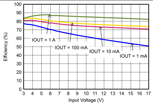
Figure 19. Efficiency With 1.25 MHz
