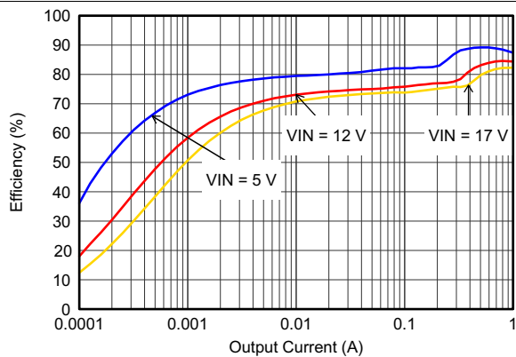
Figure 18. Efficiency With 1.25 MHz
