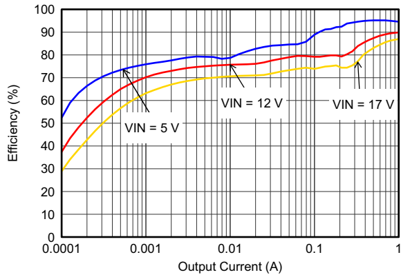
Figure 16. Efficiency With 2.5 MHz
