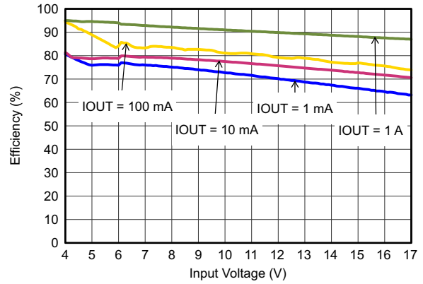
Figure 17. Efficiency With 2.5 MHz
