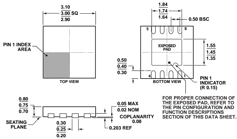
Figure 26. 8-Lead Lead Frame Chip Scale Package [LFCSLP_WD] 3 mm x 3 mm Body, Very Very Thin, Dual Lead (CP-8-13) Dimensions shown in millimeters
