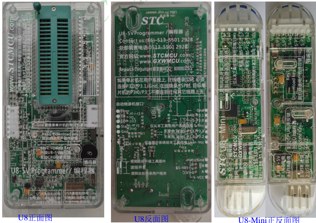
U8-Mini正反面图
