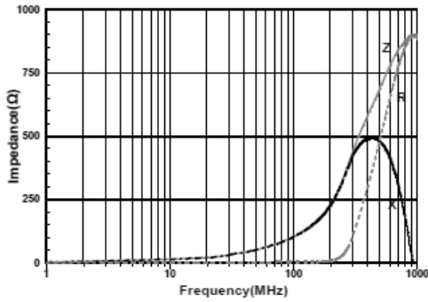
SBH1608S221MSP
