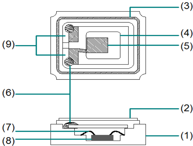
Reference drawing
