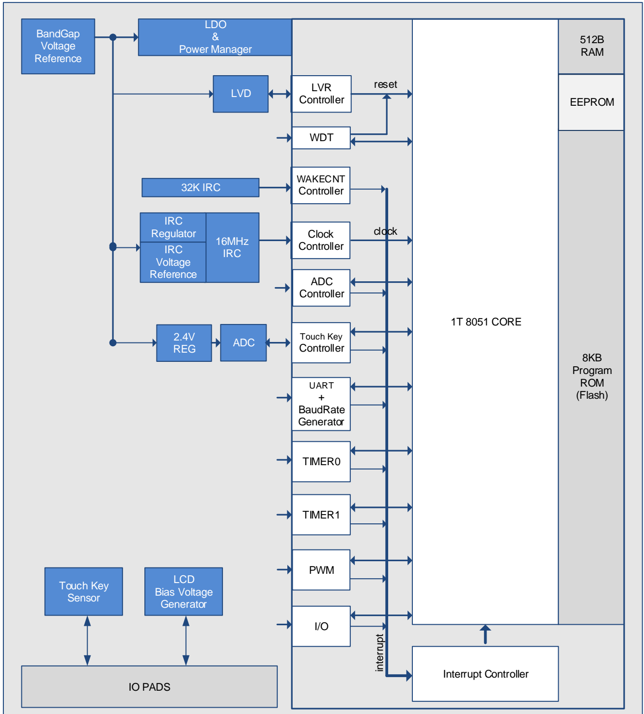
SC91F8311 BLOCK DIAGRAM
