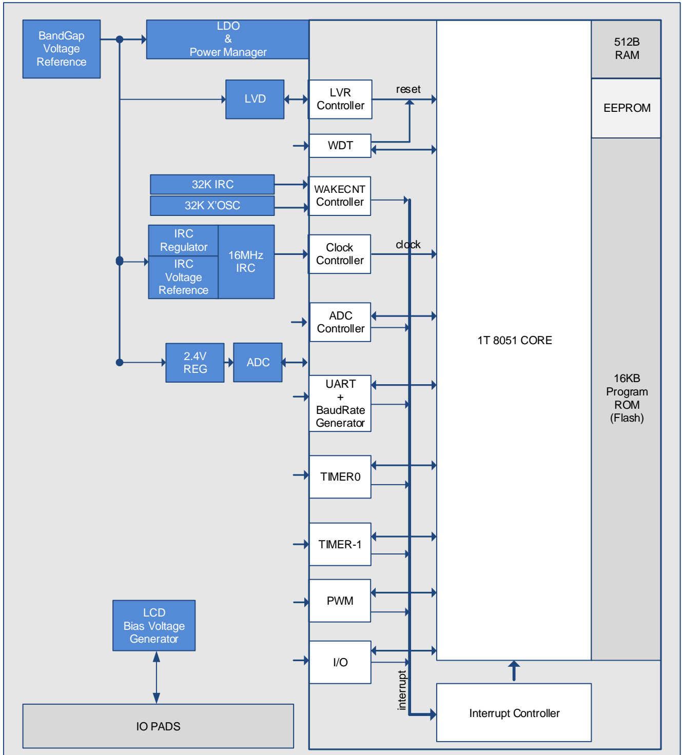
SC91F744 BLOCK DIAGRAM
