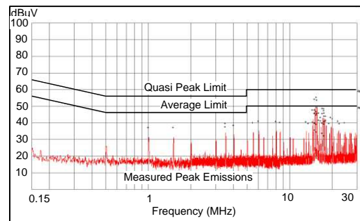
Figure 24. Conducted EMI Curve V_{OUT} = 5\text{ V} F_S = 500\text{ kHz} I_{OUT} = 1\text{ A} Measured on LM46001PWPEVM with L = 27\text{ }\mu\text{H} , C_{OUT} = 66\text{ }\mu\text{F} , C_{FF} = 33\text{ pF} . EVM input filter L_{in} = 1\text{ }\mu\text{H} C_d = 47\text{ }\mu\text{F} C_{IN4} = 68\text{ }\mu\text{F}
