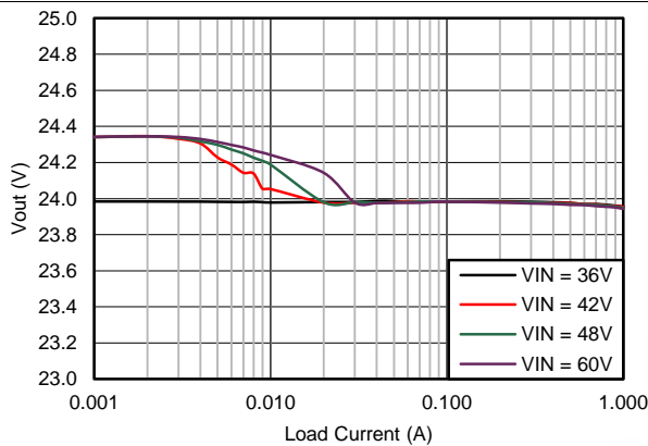
Figure 79. Output Voltage Regulation
