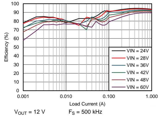
Figure 72. Efficiency
