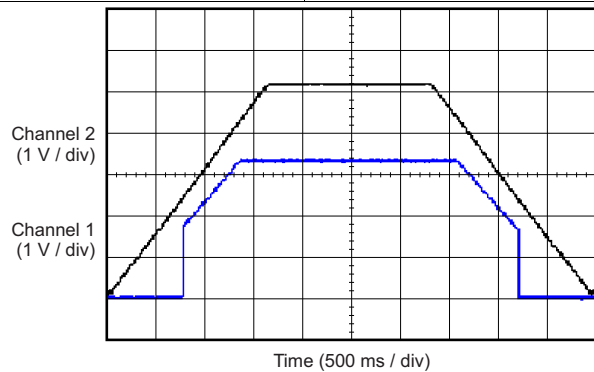
Channel 1 = V_{IN} , channel 2 = V_{OUT} , I_{OUT} = 150\text{ mA} , TPS70633
