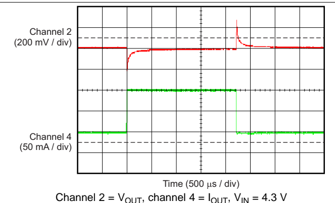
Figure 34. TPS70933-Q1 Load Transient (50 mA to 150 mA)
