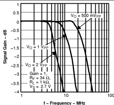
Figure 20. Frequency Response
