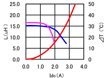
CDRH70D45BT150NP-150MC
