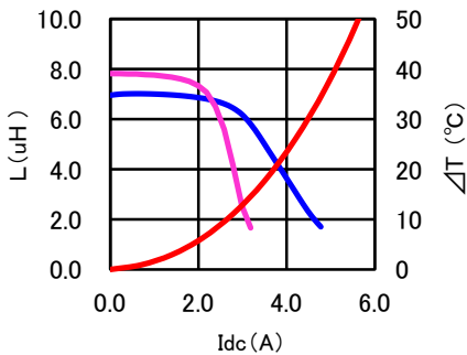
CDRH70D45BT150NP-6R8NC
