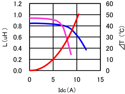
CDRH70D45BT150NP-2R2NC
