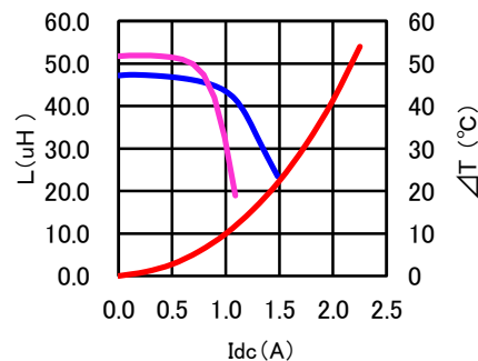
CDRH70D45BT150NP-151MC
