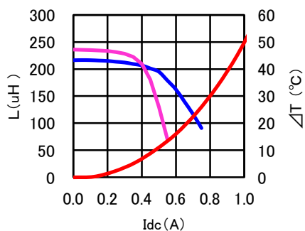
CDRH70D45BT150NP-221MC
