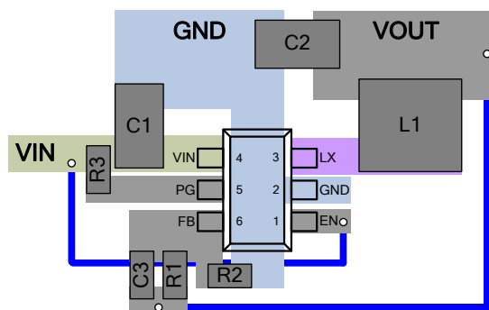
Figure 19. Recommended Layout Diagram
