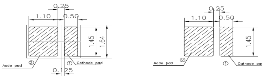
Soldering patterns
