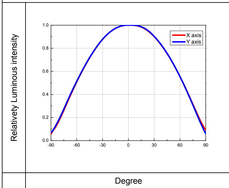
Typical Radiation Patterns
