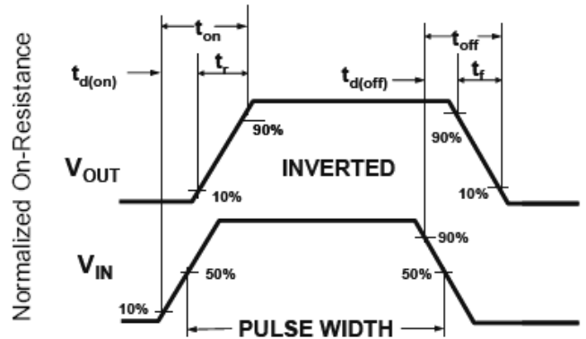
Figure 2 Switching Waveforms
