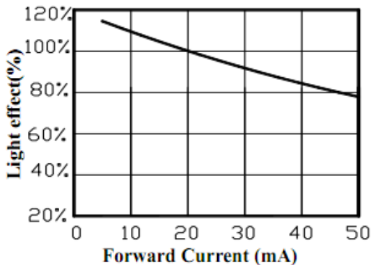
7).Relative Emission Efficiency. Current
