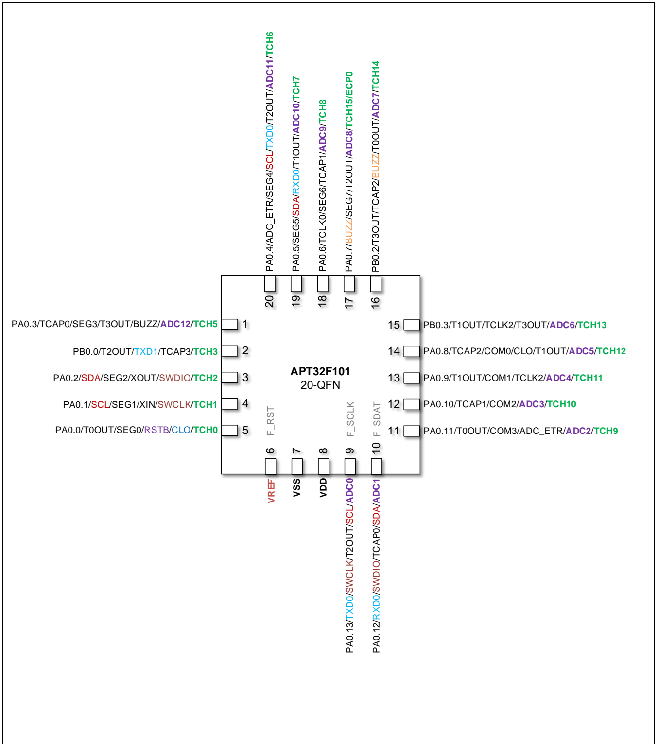
Figure 2-4 管脚定义图(20QFN-2)
