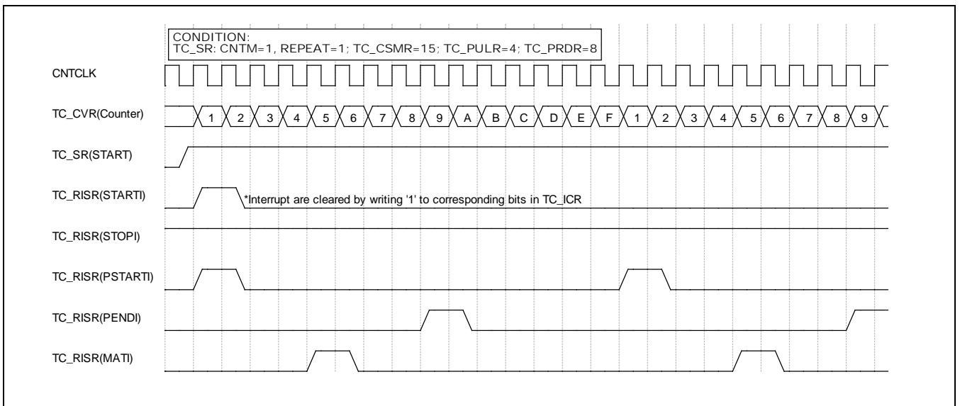
Figure 10-2 匹配和溢出时序
