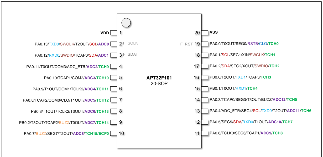
Figure 2-2 管脚定义图(20SOP)
