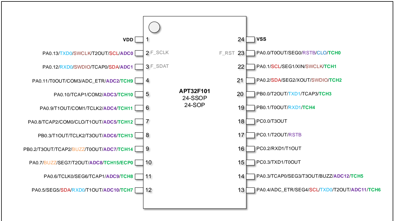
Figure 2-1 管脚定义图(24SOP/SSOP)
