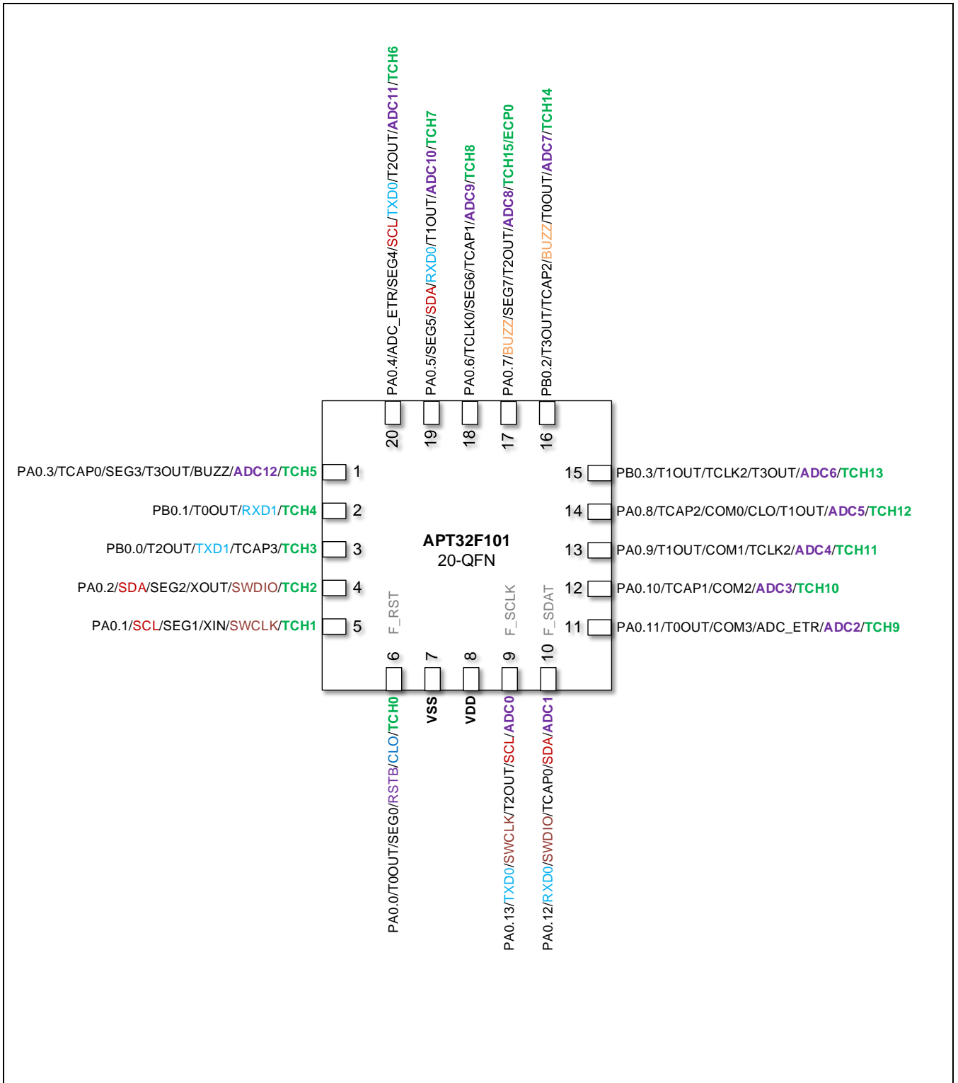
Figure 2-3 管脚定义图(20QFN-1)
