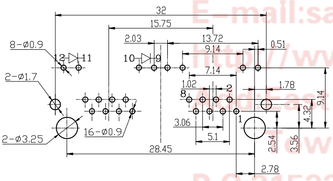
PC BOARD LAYOUT THICKNESS=1.6mm
