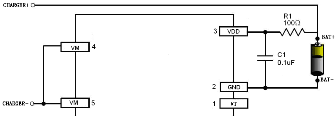
Fig 6 XB5358A in a Typical Battery Protection Circuit
