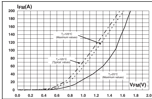
Figure 12. Forward voltage drop versus forward current (per diode)
