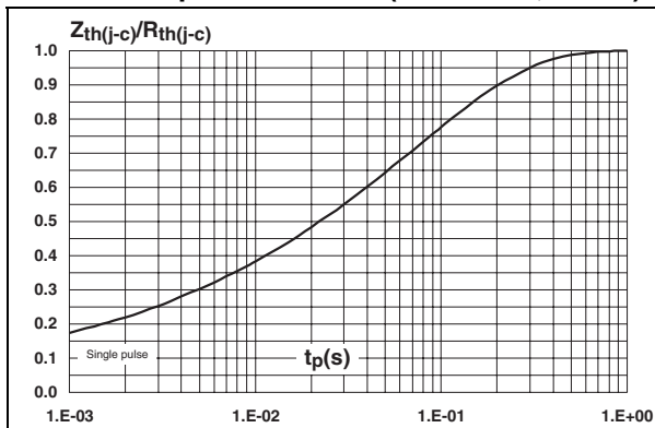
Figure 8. Relative variation of thermal impedance junction to case versus pulse duration (TO-220AB, I²PAK)
