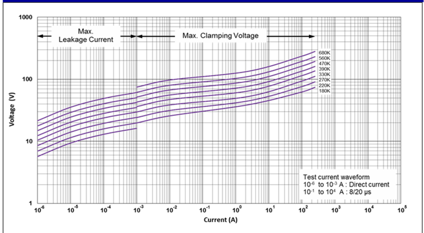
CW-07D180K to CW-07D680K V-I Curves μ
