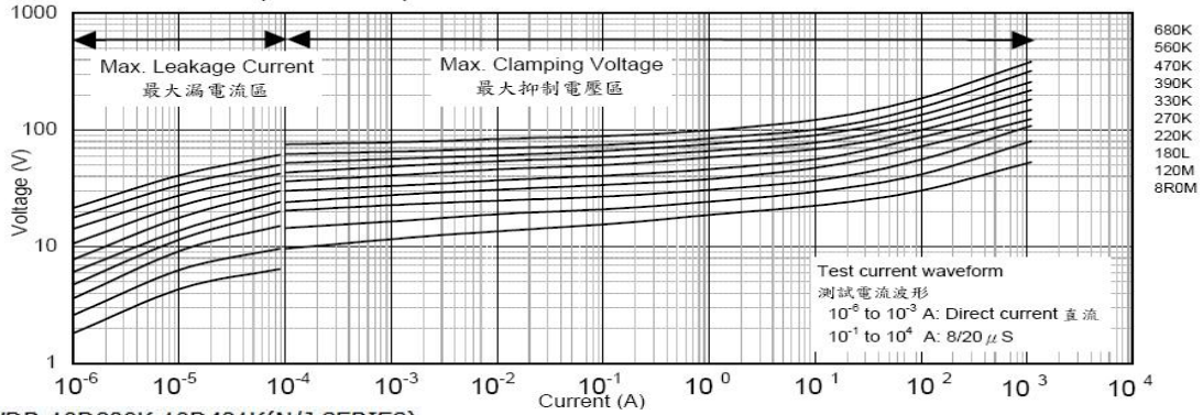
VDR-10D820K-10D431K(N/J SERIES)
