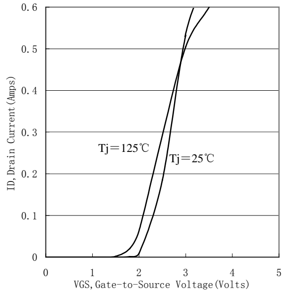
Figure 2. Transfer Characteristics
