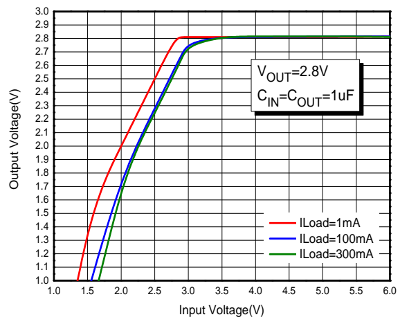
V OUT Vs. V IN
