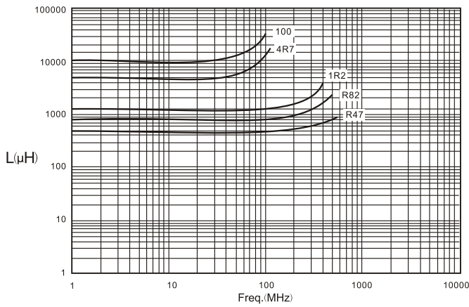
L vs Freq Plot
