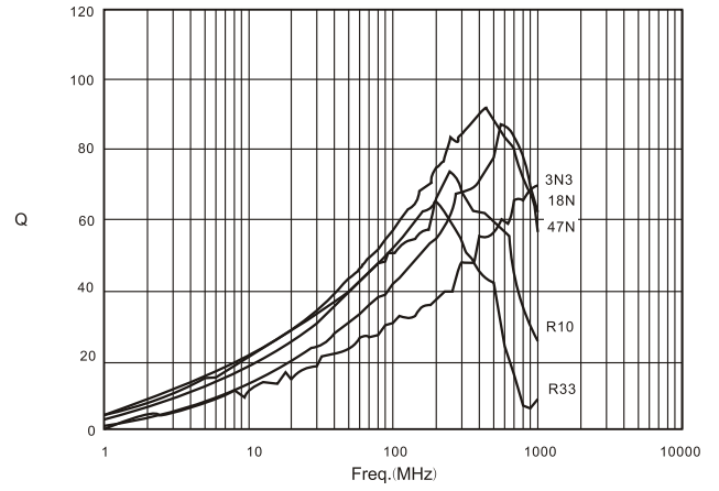
Q vs Freq Plot
