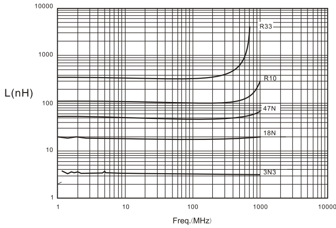
L vs Freq Plot
