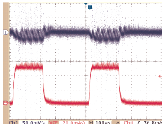
HT7737 Load Transient Response (L=100µH, C OUT =100µF, V IN =2.22V)
