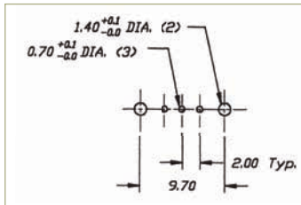
P.C. MOUNTING
