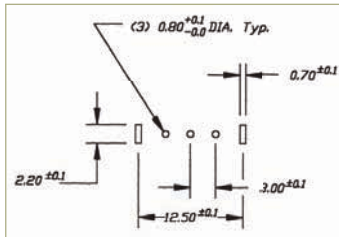
P.C. MOUNTING
