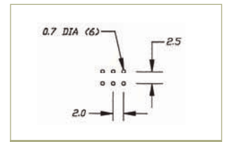
P.C. MOUNTING
