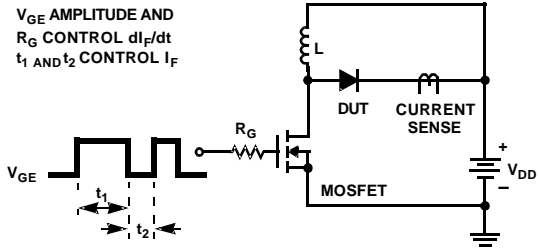
Figure 12. Test Circuit
