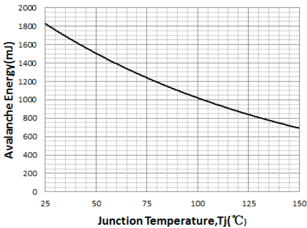
Avalanche Energy vs. Temperature
