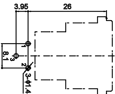
PCB LAYOUT (VIEWED FROM COPPER SIDE)
