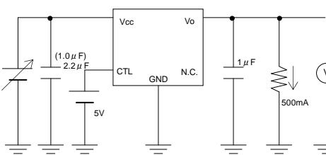
Measurement Circuit of Fig.4 and Fig.16
