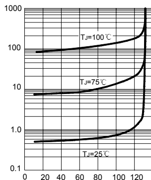
FIG.6 – TYPICAL REVERSE CHARACTERISTICS
