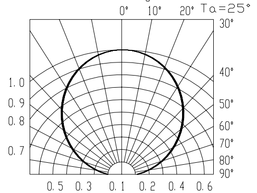
Radiation Diagram
