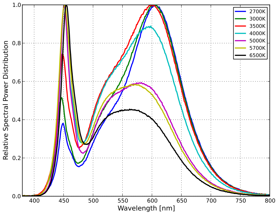
Figure 1b. Typical normalized power vs. wavelength for L130-xx80001400001 at 60mA, T_j=25^{\circ}\text{C} .
