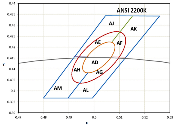
Figure 7a. Color bin structure for LUXEON 3014 2200K, hot-color targeted at T_j=65^\circ\text{C} .
