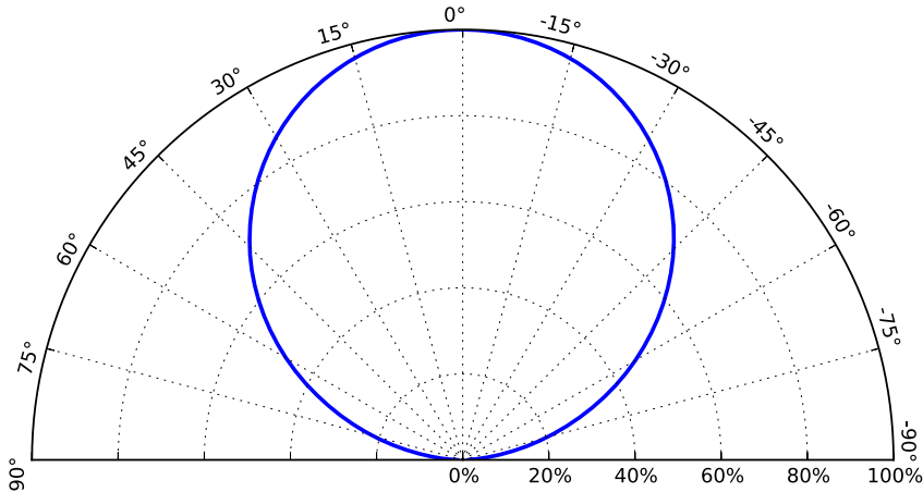
Figure 5. Typical polar radiation pattern for L130-xxxx001400001 at 60mA, T J =25°C.
