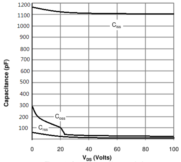
Figure 8: Capacitance Characteristics
