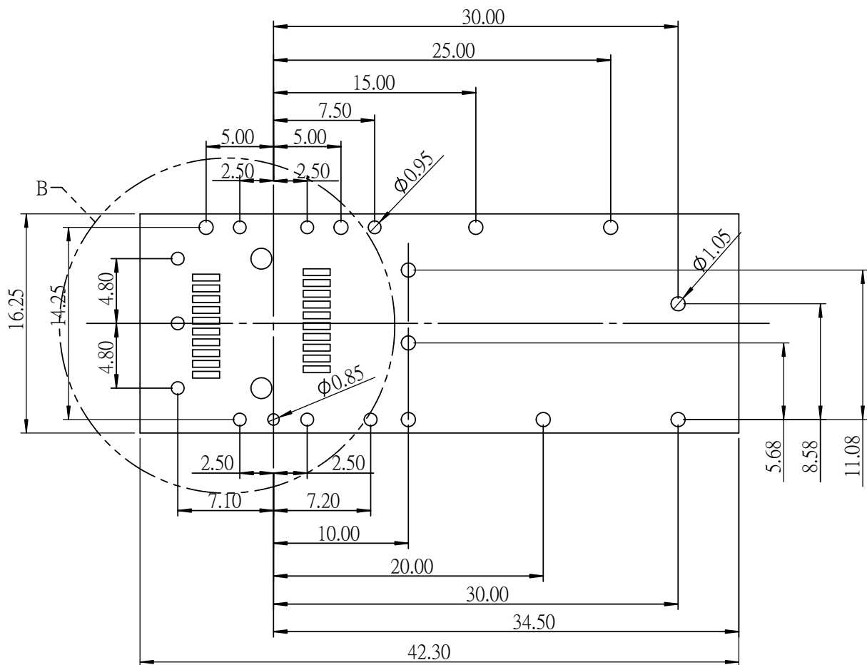
PCB LAYOUT
