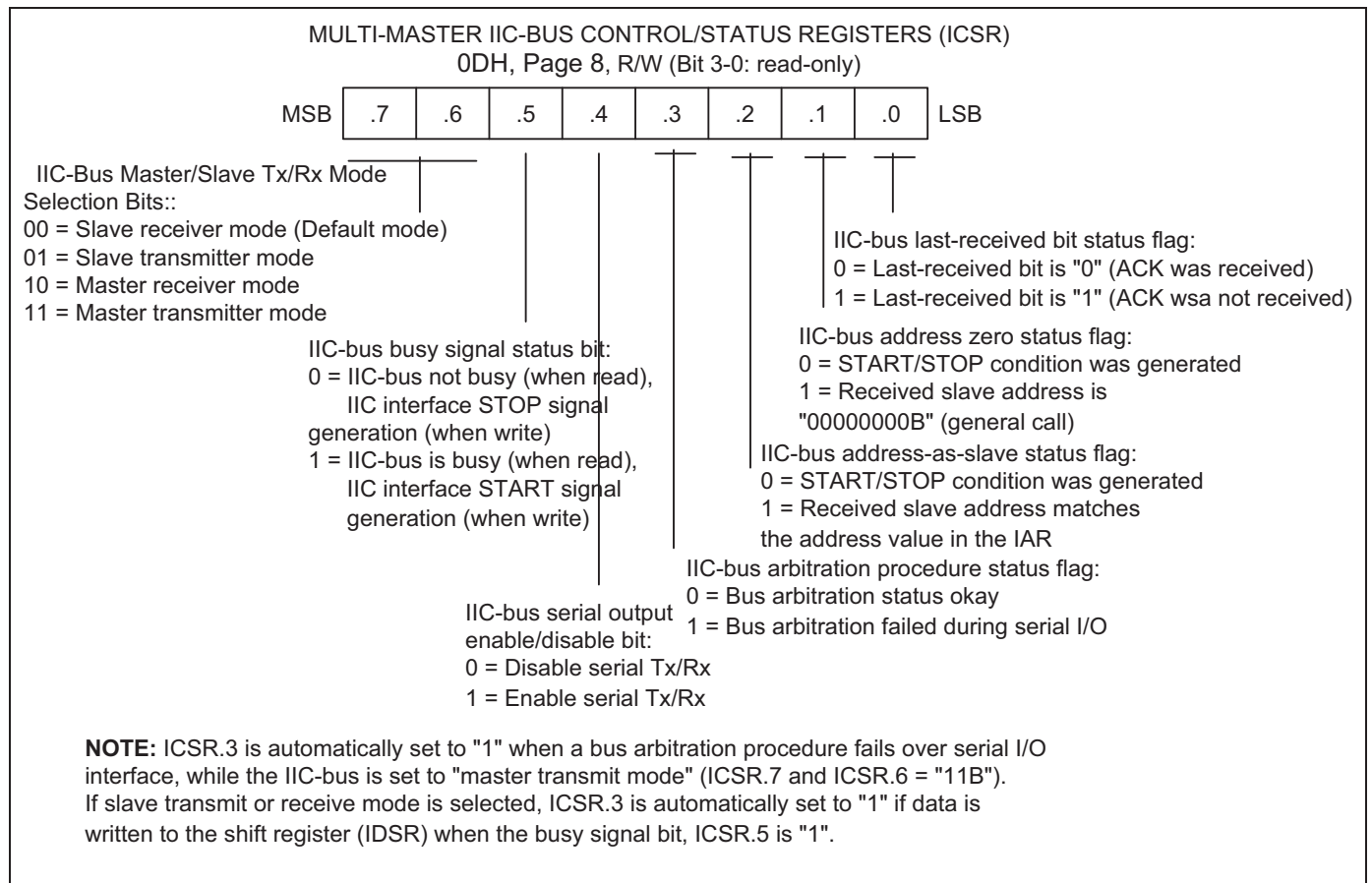
Figure 18-2 Multi-Master IIC-Bus Control/Status Register (ICSR)
