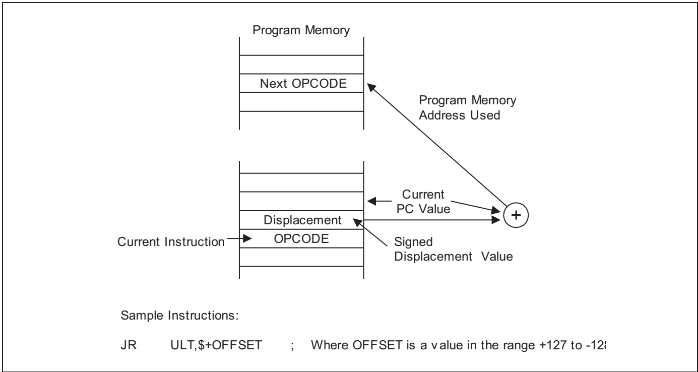
Figure 3-13 Relative Addressing
