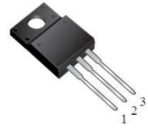
ITO-220AB PS30U60FCT
