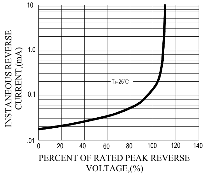
FIG.4-TYPICAL REVERSE CHARACTERISTICS
