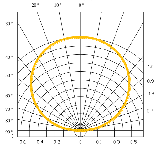
Radiation Diagram 辐照图
