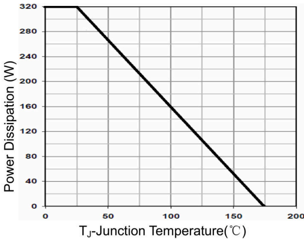
Figure 9 Power De-rating
