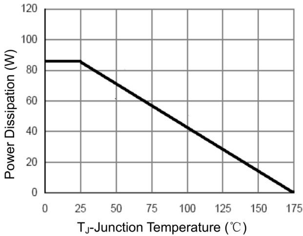
Figure 9 Power De-rating
