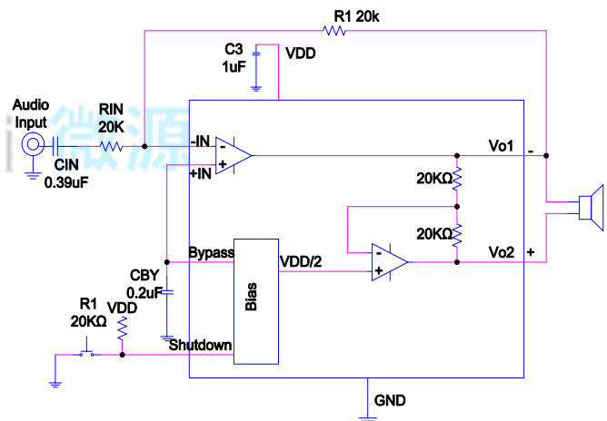
Figure 1. Single Input
