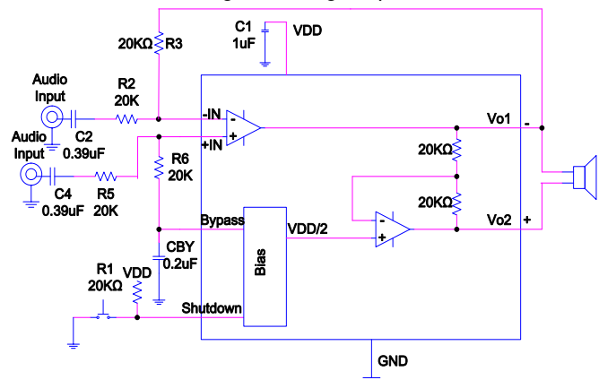
Figure 2. Differential Input
