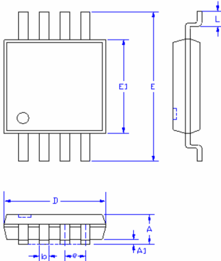
MSOP-8
