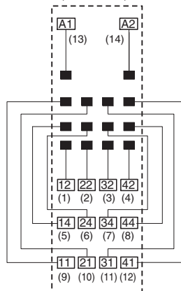
Terminal Arrangement/ Internal Connection Diagram (TOP VIEW)
